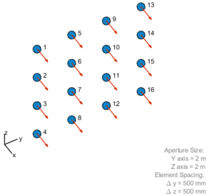
Array Geometry
